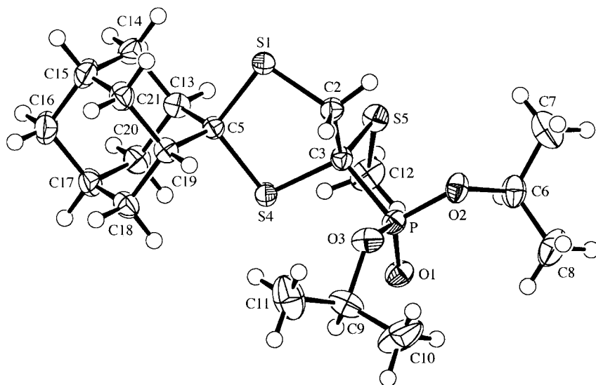
Figure 3. ORTEP plot [11] of the molecular structure of 20 (50% probability ellipsoids).
