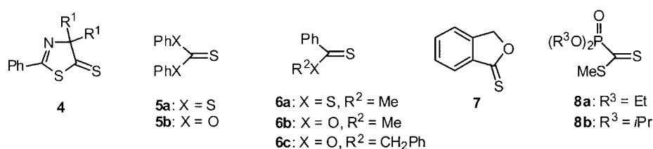
Figure 1. Thiocarbonyl compounds as dipolarophiles.
