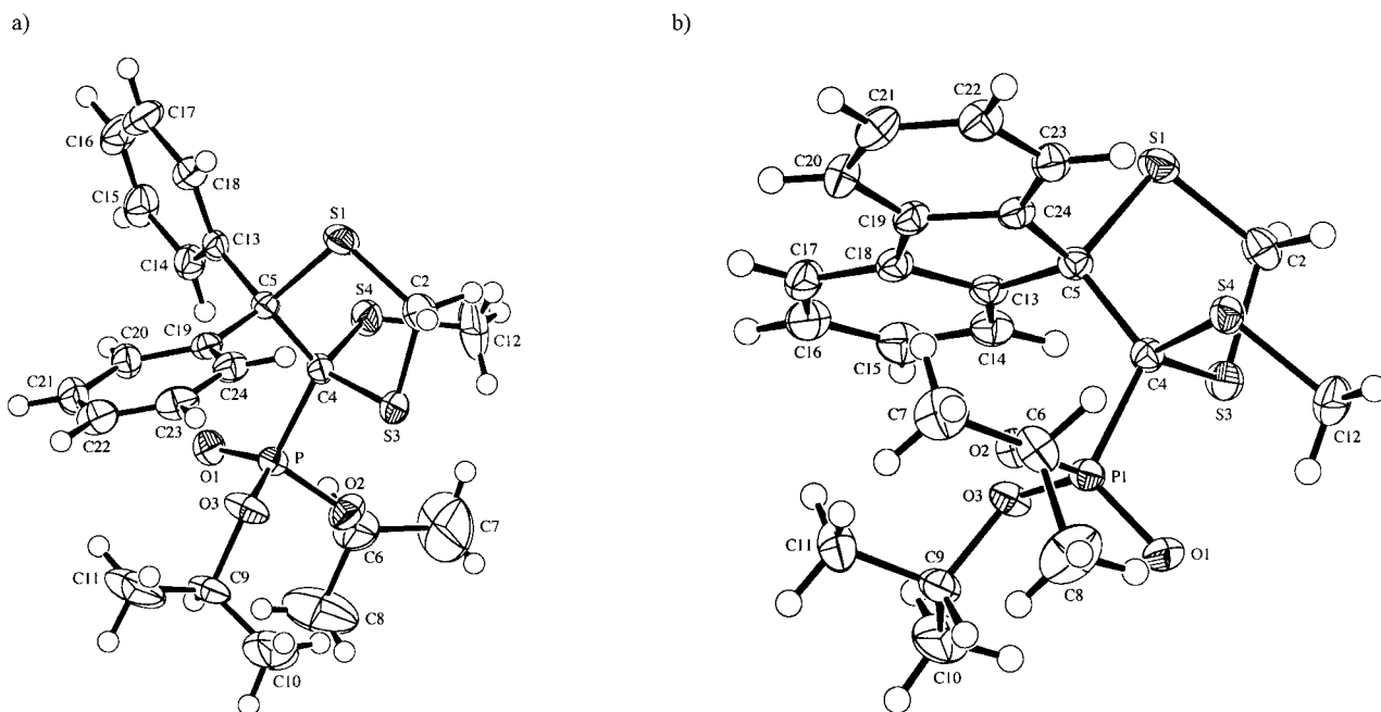
Figure 4. ORTEP plots [11] of the molecular structures of: a) 21b and b) one of the two symmetry-independent molecules of 22b (50% probability ellipsoids).
