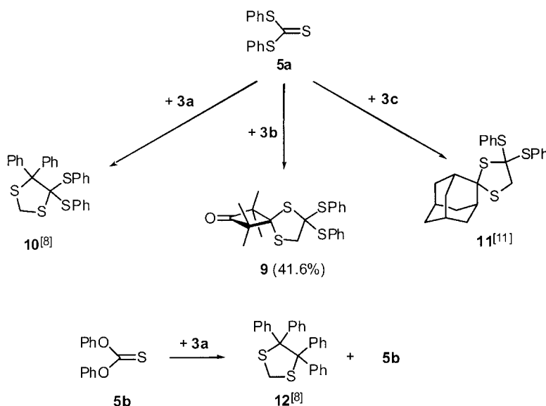
Scheme 2. Reactions of thiocarbonyl ylides 3 with trithiocarbonate 5a and thiocarbonate 5b .
