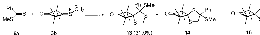
Scheme 3. Reaction between dithioester 6a and thiocarbonyl ylide 3b .
