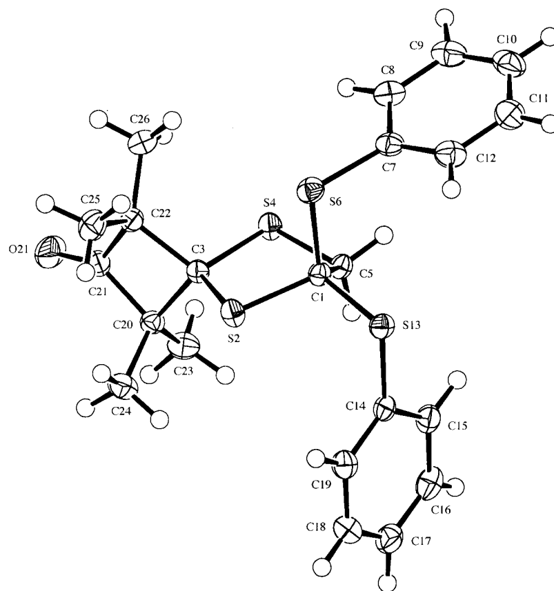
Figure 2. ORTEP plot [11] of the molecular structure of 9 (50% probability ellipsoids).
