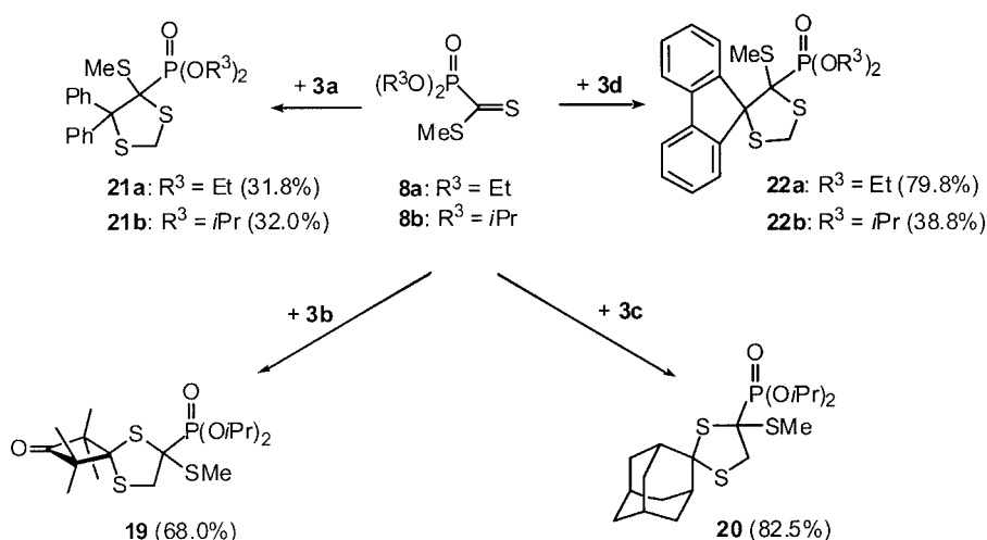
Scheme 5. Reactions of dithioesters 8 with thiocarbonyl ylides 3a–d .
