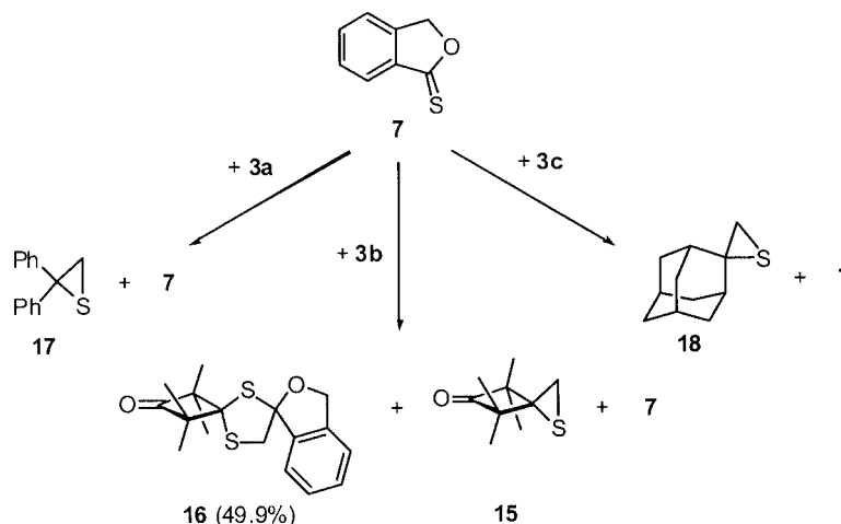
Scheme 4. Reactions of thioester 7 with thiocarbonyl ylides 3a–c .
