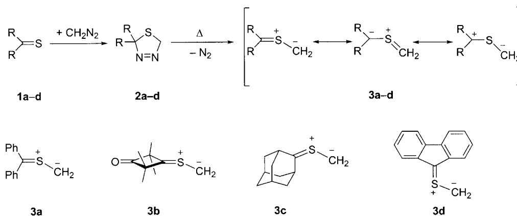
Scheme 1. Synthesis of thiocarbonyl ylides 3 .
